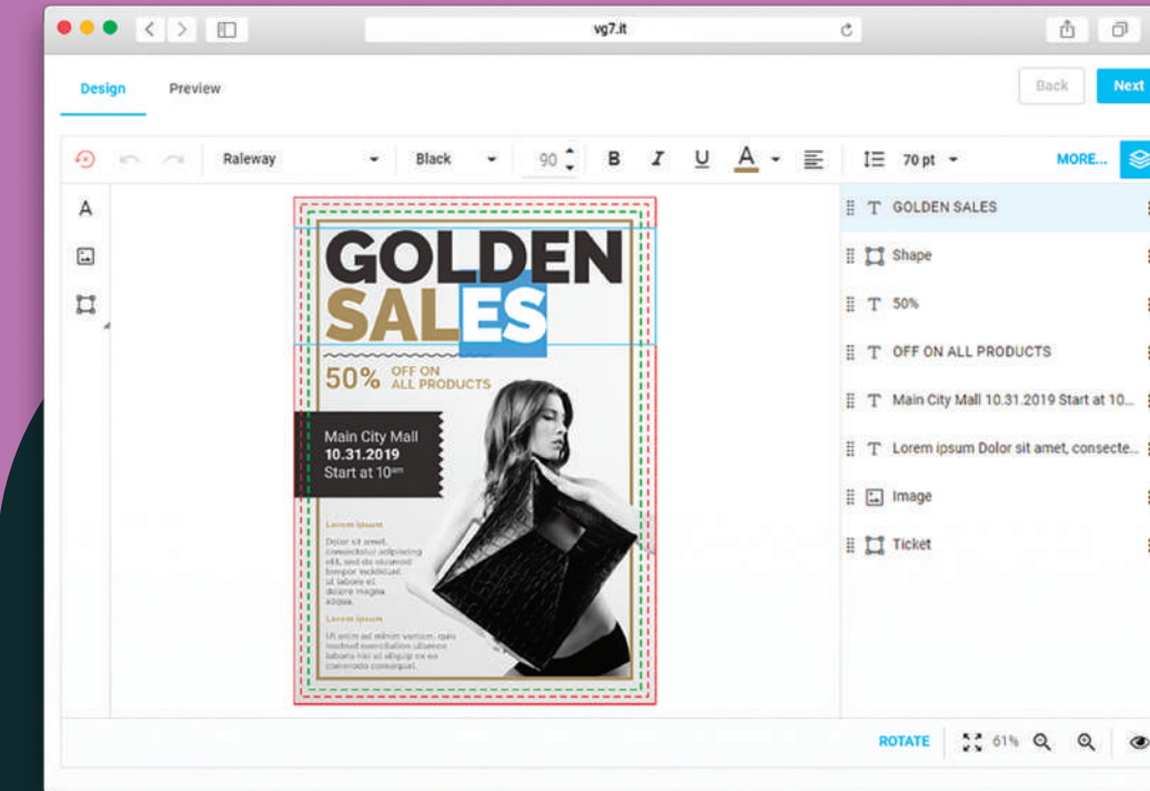
Editor configuration
